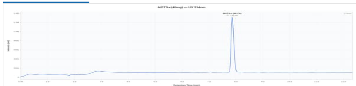
MOTS-C 40mg - MS40-20260421: UV Chromatogram
